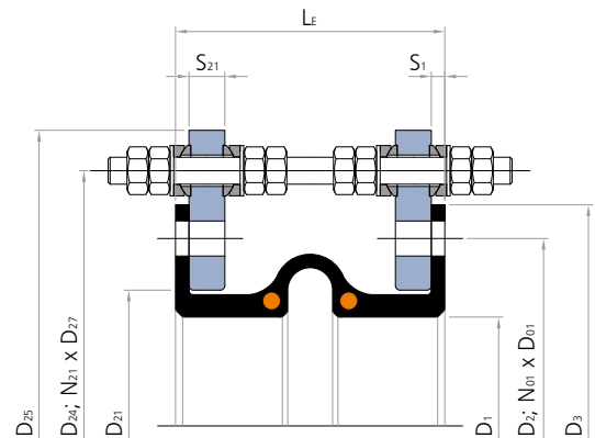
Cross section U216M
