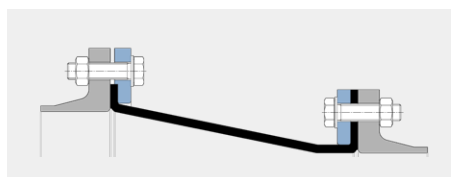
Full faced / swivel flanged combination
